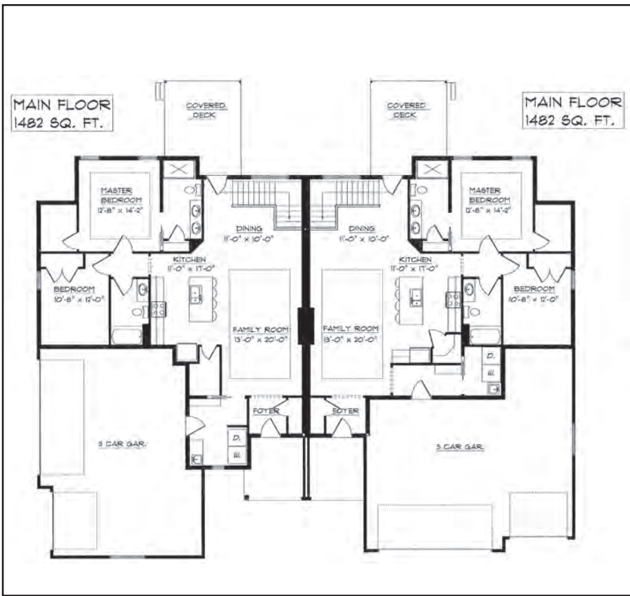
Main Floor
