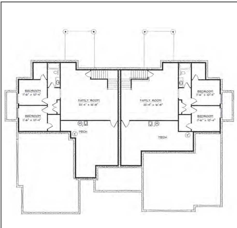
Lower Level
