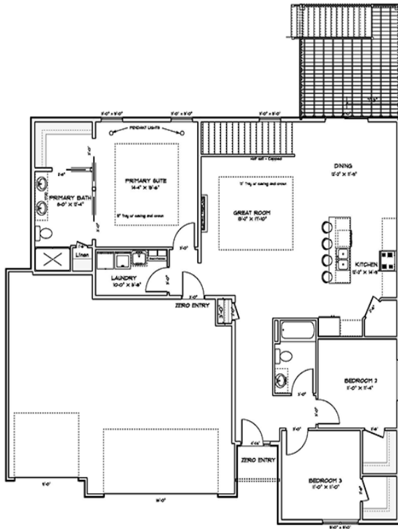
MAIN FLOOR - 1648 SF
