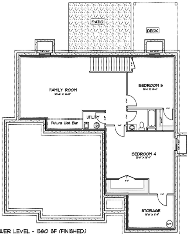
LOWER LEVEL - 1380 SF (FINISHED) 1648 SF (TOTAL AREA)
