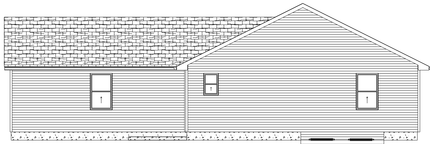
Rear Elevation
